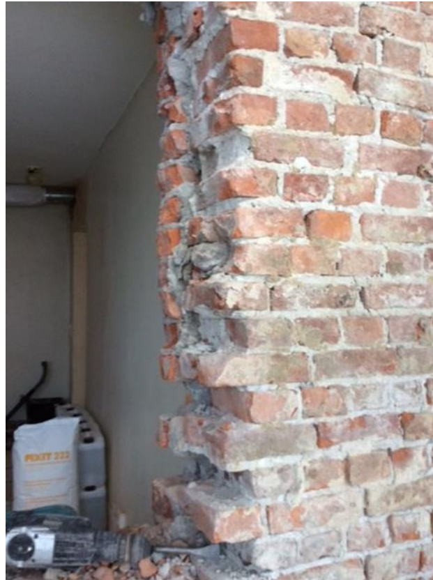
Figure 21 - Picture showing a window cavity after cleaning, before application of FIXIT (source: Boligbygg).
