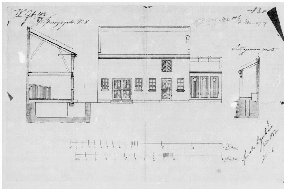
Figure 19: Architectural drawing of the building anno 1887 (Source: Boligbygg).
