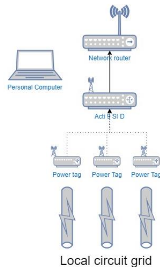
Figure 9- Example of Acti 9 Smartlink system setup connected to the local grid.
