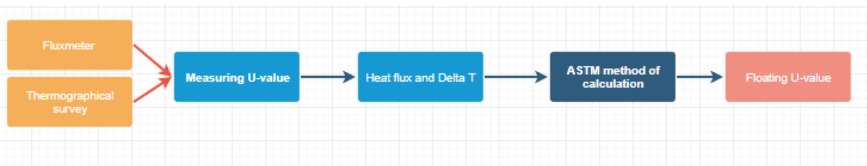
Figure 4- Figure describing the methodical approach to determining U-value through measurements.
